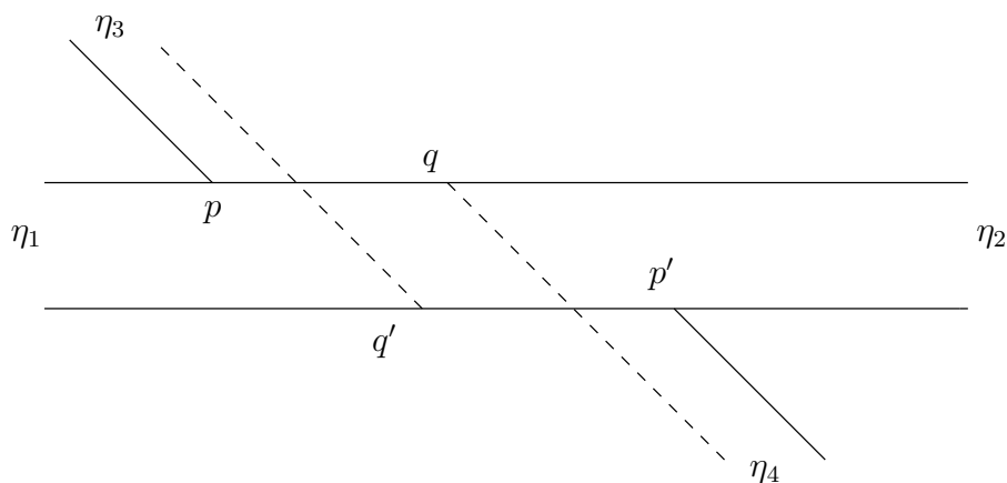
Figure III.4: The situation from Lemma III.3.7. Observe that q, q' are not tripodal points (unless q = p' and q' = p ).
